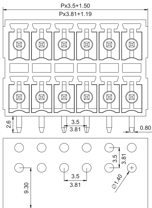
KF2EDGKRH-3.5/3.81
