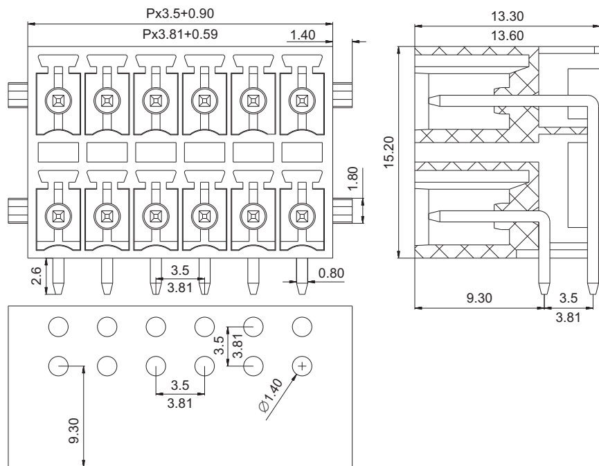
KF2EDGKRG-3.5/3.81
